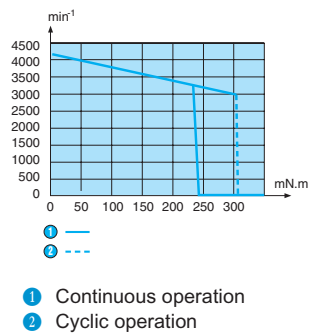
Speed/torque
