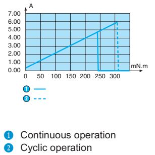
Current/torque
