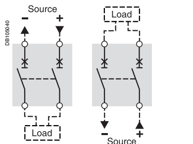
Upstream/downstream connections to top or bottom connectors.
