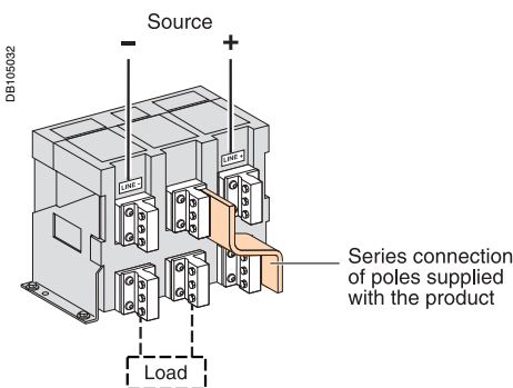
Masterpact NW - supplied ready for installation (here with vertical rear connections).
