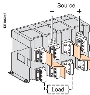
Rear view with connections.
