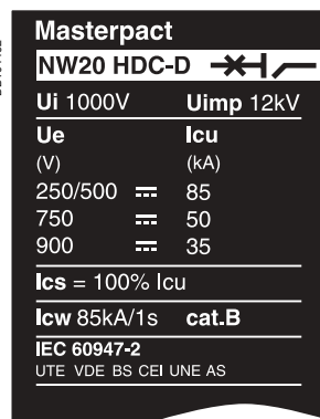
NW20 HDC-D rating plate.
