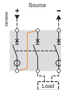
Three-pole case - three poles in series (front view).
