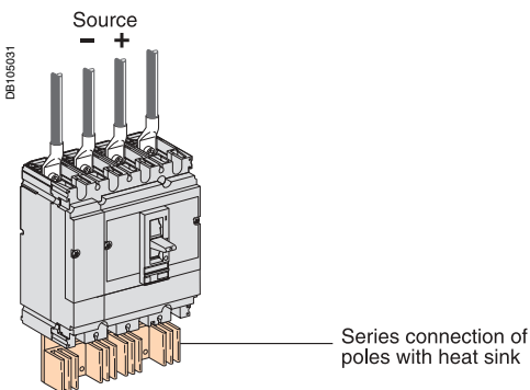
Compact NS - safety and flexibility.
