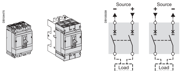
All connections are possible for the fixed and withdrawable versions.
