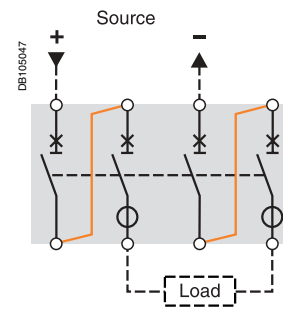
Four-pole case - four poles in series (front view).
