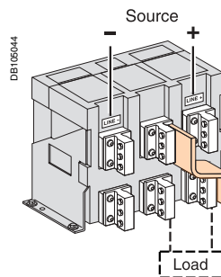
Rear view with connections.
