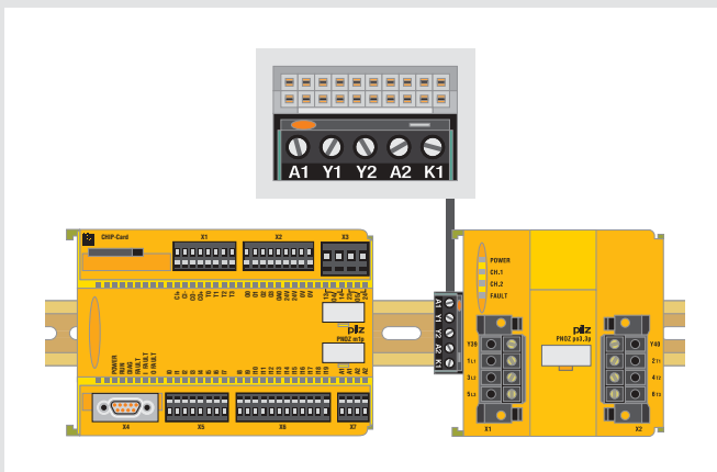
Combine the PNOZpower and PNOZmulti modular safety systems easily using the coupling connector PNOZ pe2p.
